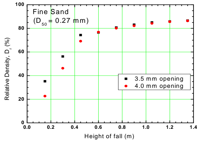
Figure 7: Relative Density vs. height of fall plot for fine sand.
