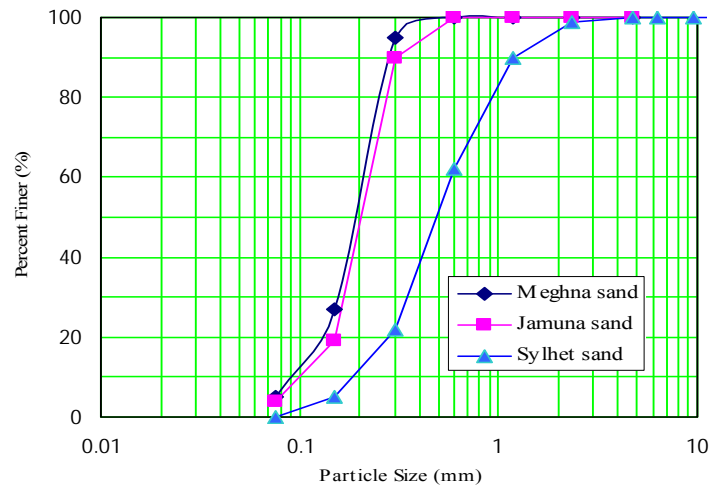
Figure 5: Grain size distribution of sands used in the study.
