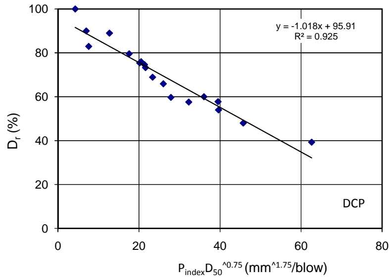
Figure 12: Correlation between Relative Density and P_{index}D_{50}^{0.75} for DCP
