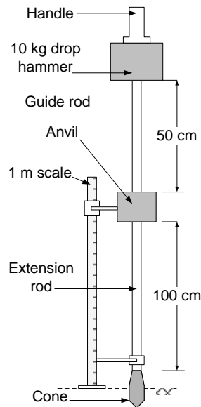
Figure 1: Schematic diagram showing arrangement for test with Dynamic Probing Light (DPL)
