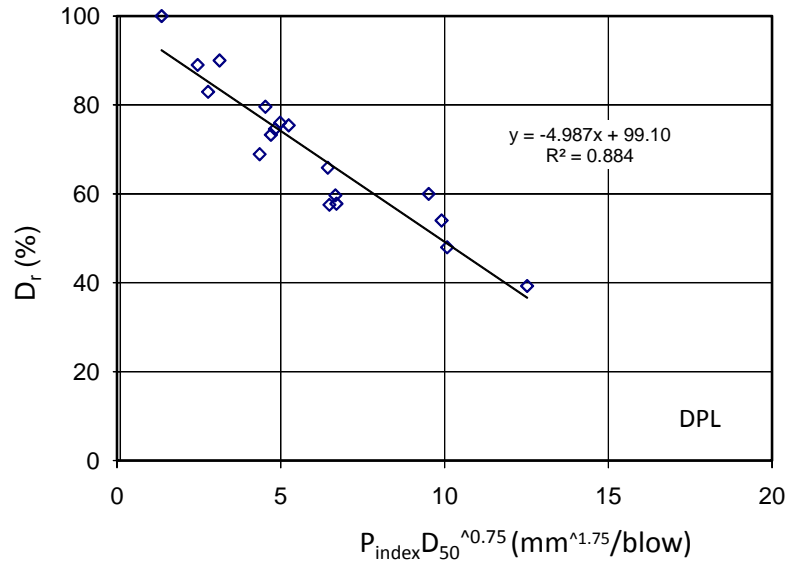
Figure 13: Correlation between Relative Density and P_{index} D_{50}^{0.75} for DPL.
