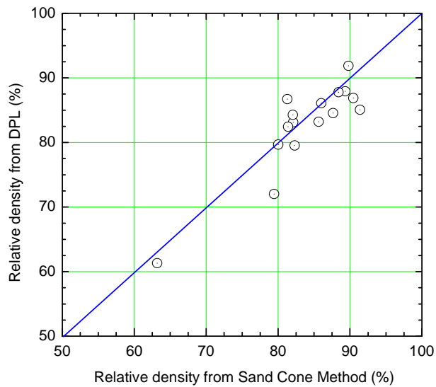
Figure 16: Comparison of Relative Density obtained from DPL test and Sand Cone Method after incorporation of correction factor
