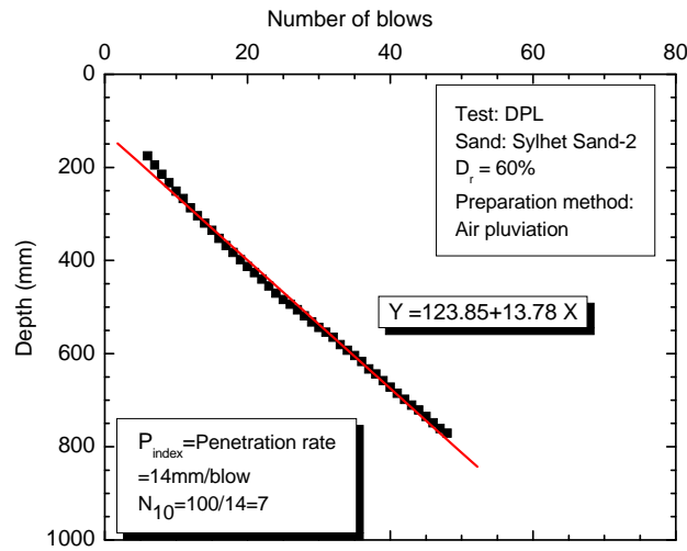
Figure 9: Typical plot of number of blows vs. depth (DCP) for fine sand in calibration chamber
