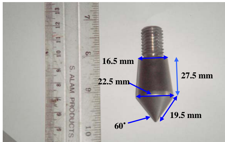
Figure 4: Dimensions of probing cone of DCP
