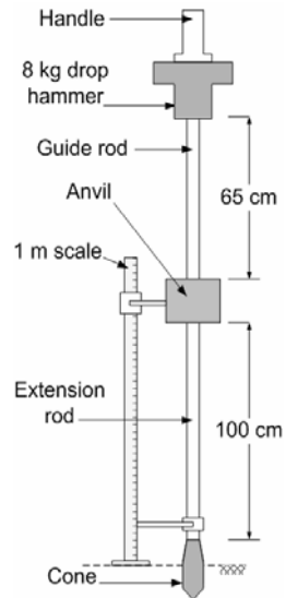
Figure 3: Schematic diagram showing arrangement for a Dynamic Cone Penetration (DCP) test
