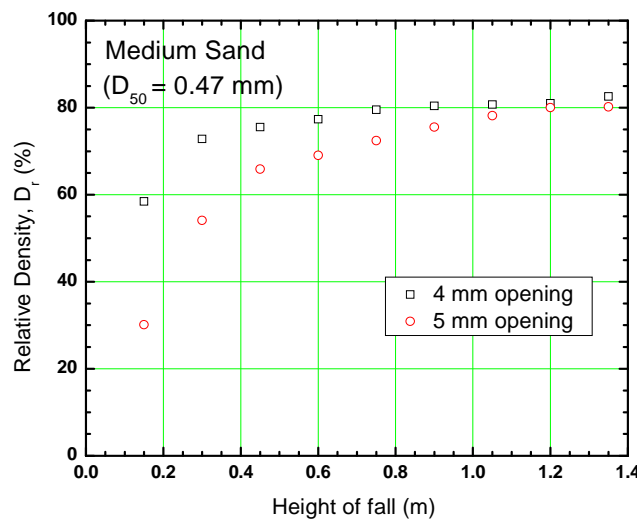
Figure 8: Relative Density vs. height of fall plot for medium sand
