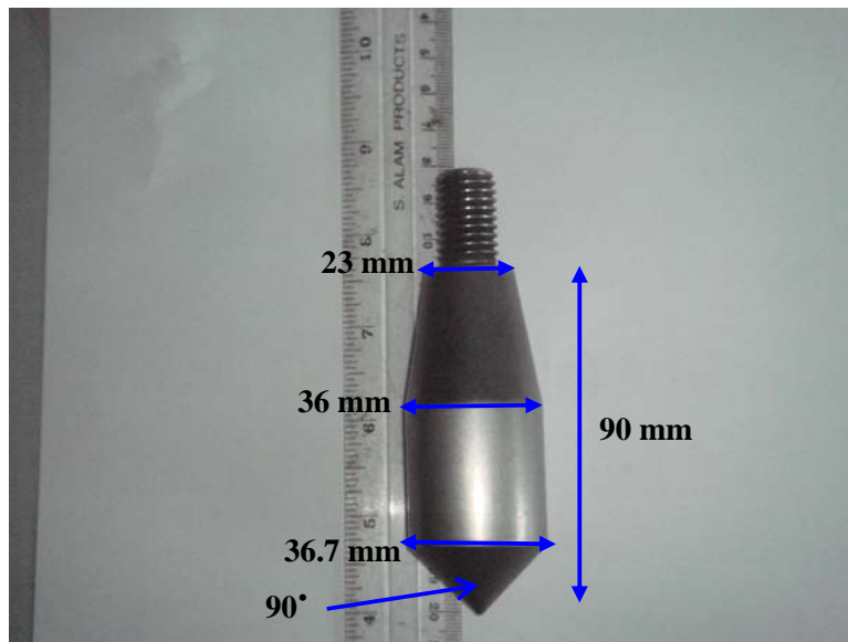
Figure 2: Dimensions of probing cone of DPL
