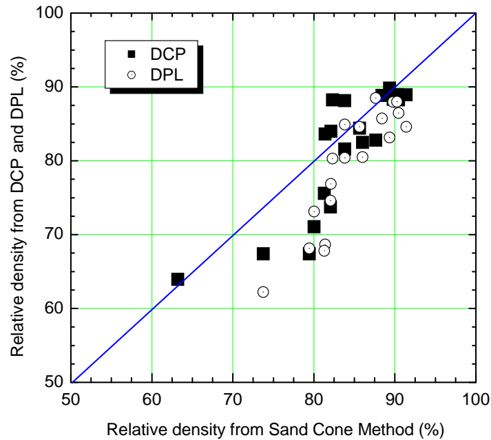
Figure 14: Comparison of Relative Density obtained from DCP and DPL test and Sand Cone Method without applying correction factor
