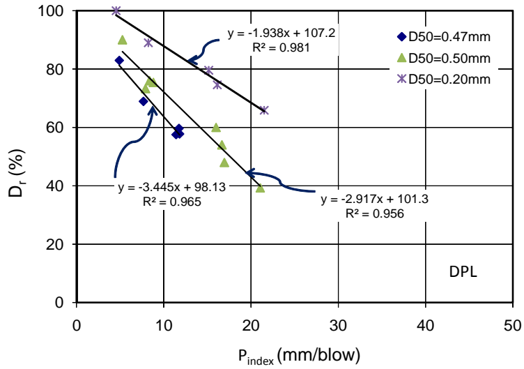
Figure 11: Correlation between Relative Density and P_{index} for DPL
