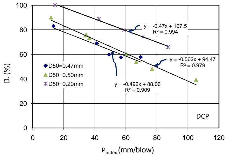
Figure 10: Correlation between Relative Density and P_{index} for DCP
