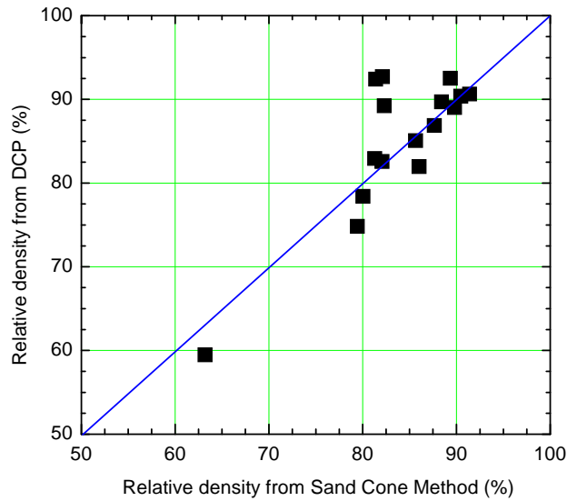
Figure 15: Comparison of Relative Density obtained from DCP test and Sand Cone Method after incorporation of correction factor
